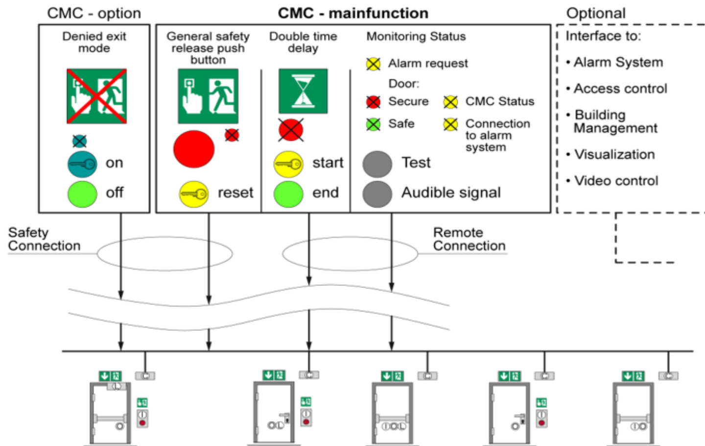
Figure 3 — Example of a CMC Control Panel
